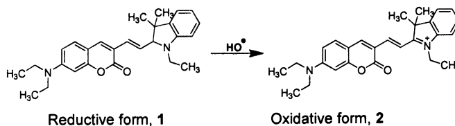
Figure 2. Ratiometric fluorescent probe with high selectivity for hydroxyl radicals.
